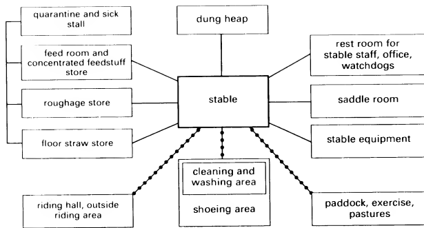
1 Function diagram of a horse stable
